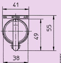
Rotary actuator, small, lockable, for 8008, assembly 734
