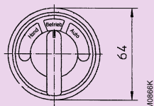
Rotary actuator, large, for 8008, assembly 731
