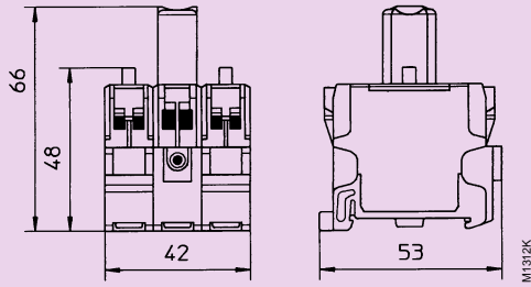
Illuminated pushbutton Assemblies 737, 738, 739
