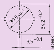
Cut-out details
