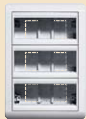
150418BA with supporting frame and cover plate (173x247x65 mm)
